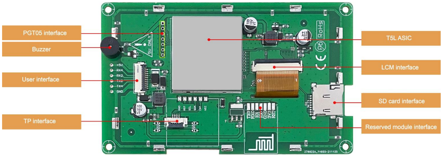
Hardware interface
