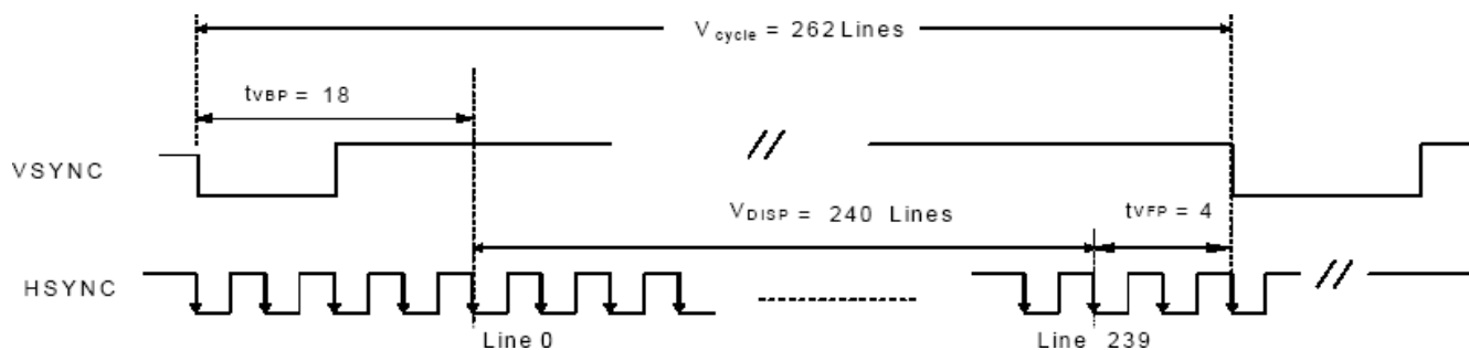
Figure 3 Data Transaction Timing in Serial RGB (8 bit) Interface (SYNC Mode)
