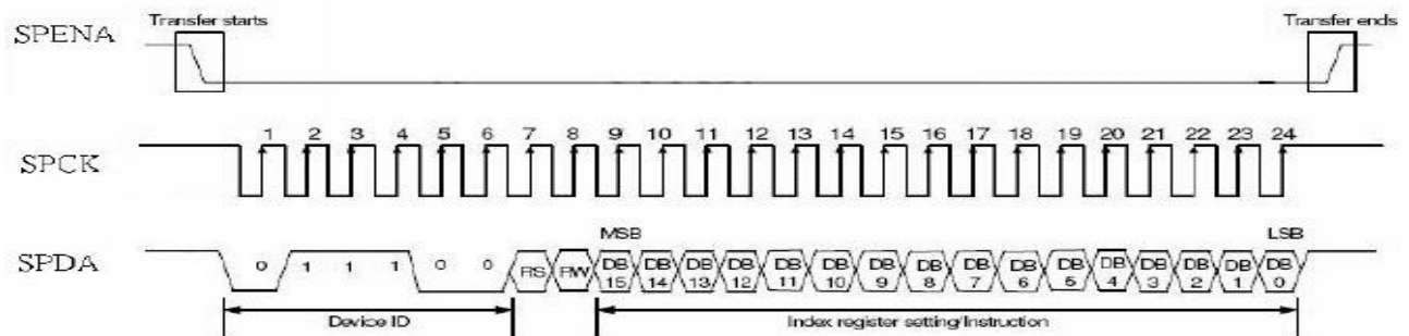
Figure12 SPI timing
